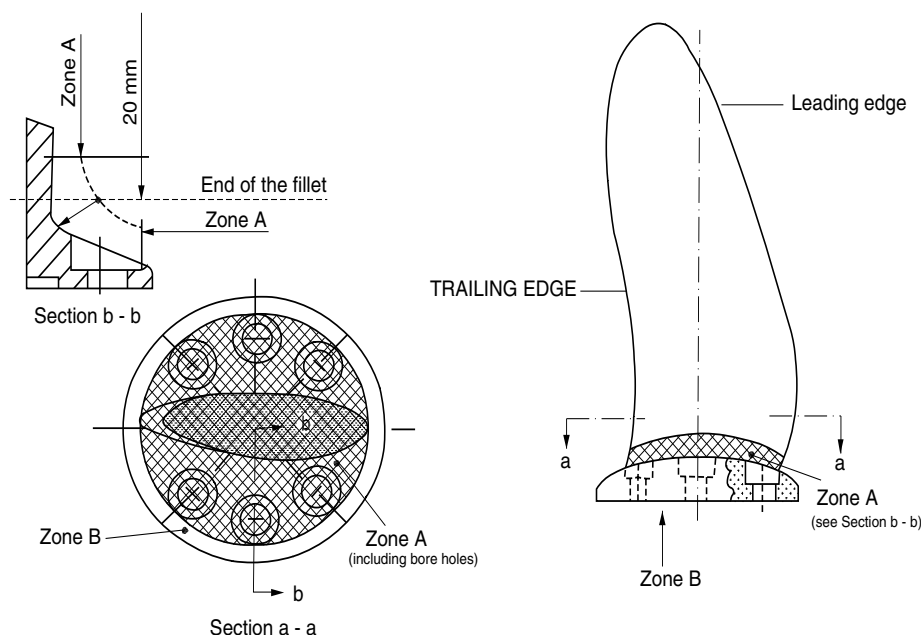
Figure 6 : Severity zones for controllable pitch and built-up propeller
