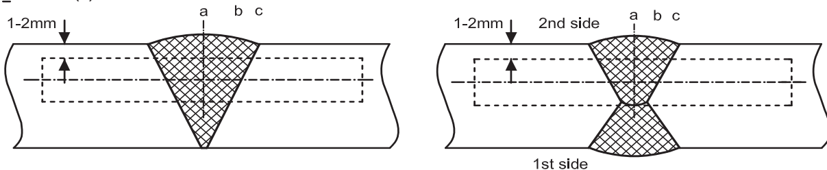
Figure 3 : Locations of V-notch for butt weld of normal heat input (heat input ≤ 50 kJ/cm)
