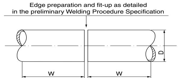
Figure 10 : Pipe weld test assembly
