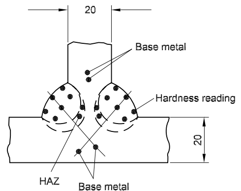
Figure 8 : Hardness readings
