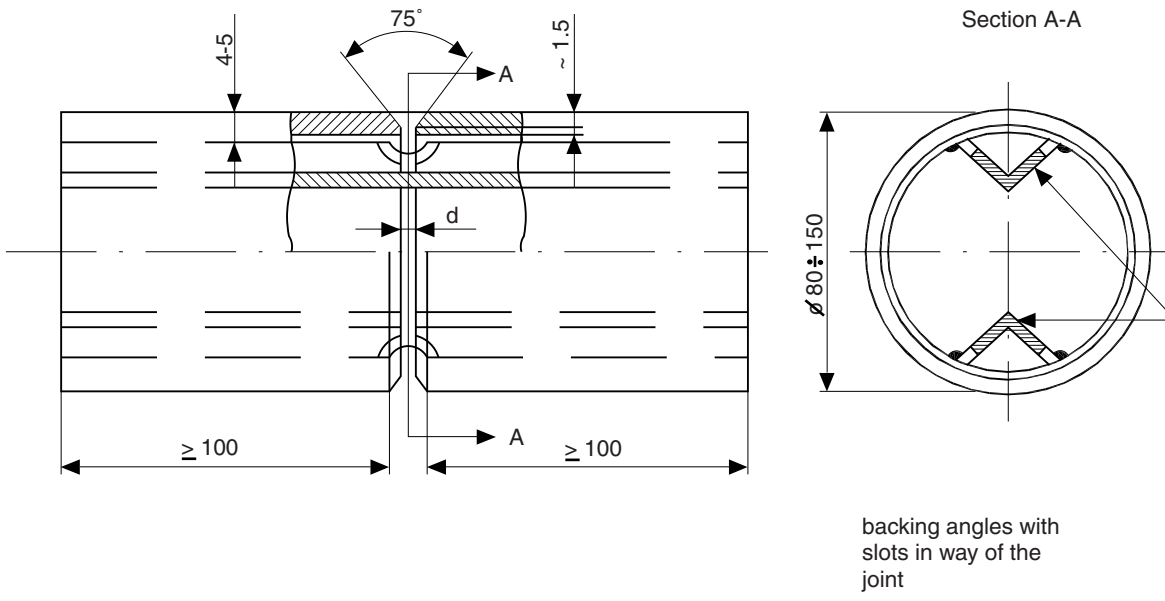
Figure 3 : Pipe assembly
