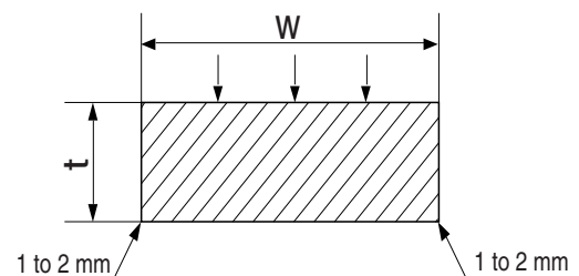
Figure 7 : Flat bend specimen
