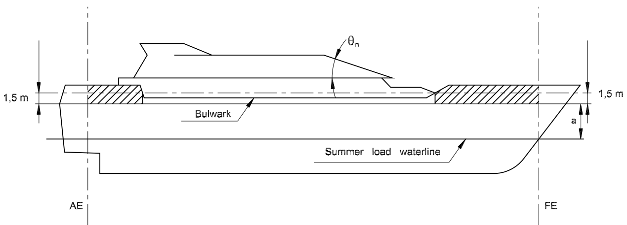
Figure 2 : Ships with inclined front bulkhead Effective area of bulwarks or fixed screen to be included in the Equipment Number
