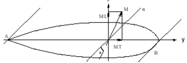
Figure 5 : Locations of max stress under combined bending
