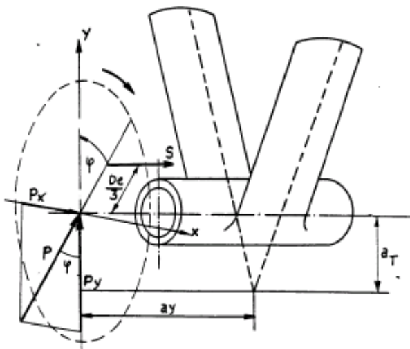
Figure 6 : Definitions of forces, directions and distances
