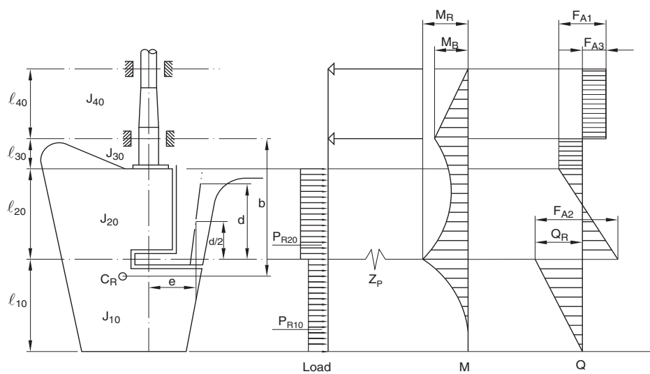
Figure 3 : 2 bearing semi-spade rudders with rudder horn
