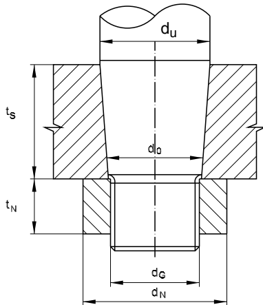
Figure 5 : Geometry of cone coupling
