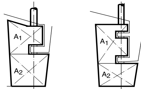
Trapezoidal rudder blade Semi-spade rudder with rudder horn - 2 bearings
