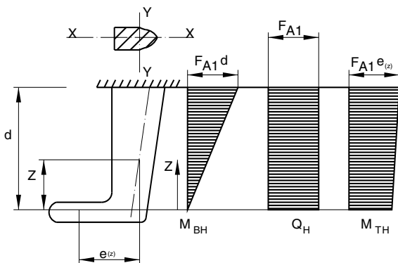
Figure 10 : Rudder horn geometry
