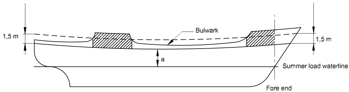
Figure 2 : Ships with inclined front bulkhead Effective area of bulwarks or fixed screen to be included in the Equipment Number
