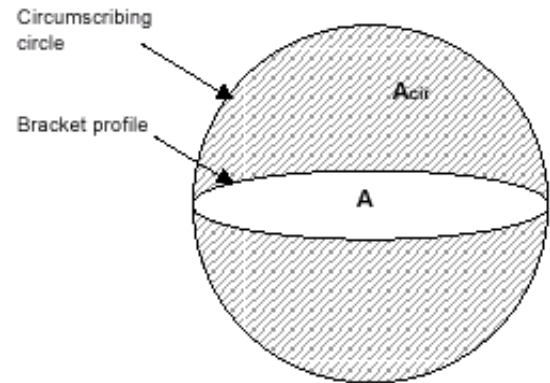
Figure 7 : Added mass of water surrounding the bracket
