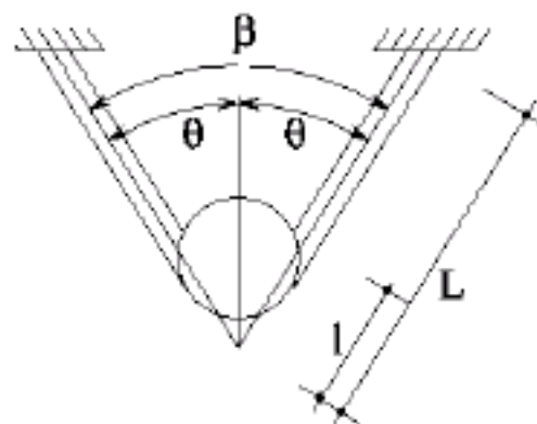
Figure 2 : Tangential type double arm propeller bracket
