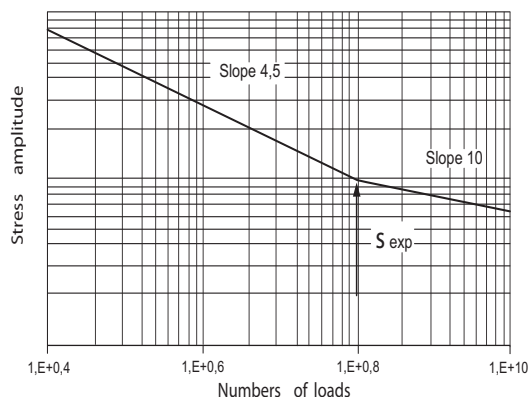
Figure 4 : Two-slope S-N curve
