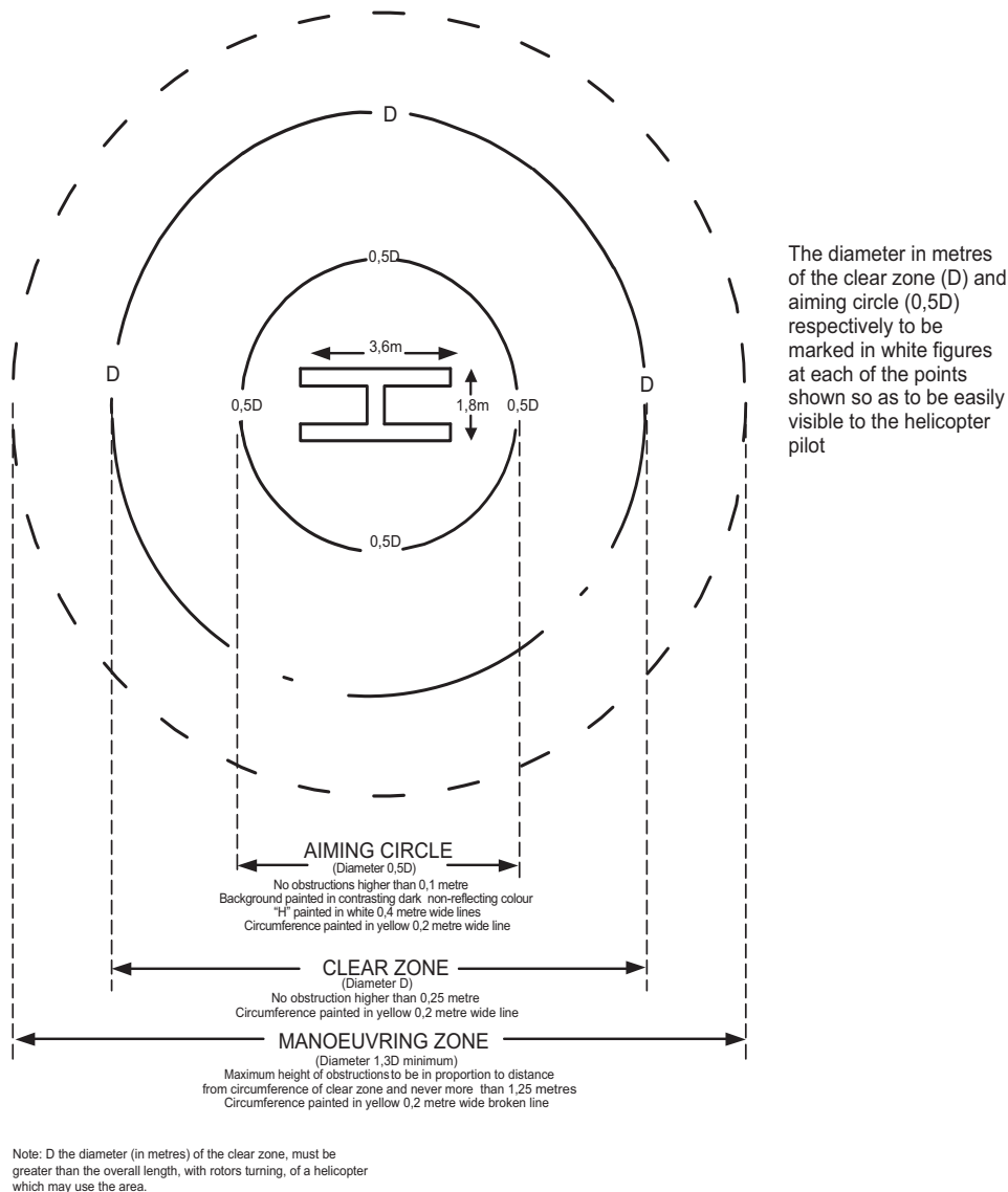
Figure 2 : Landing area without unobstructed access from ship's side
