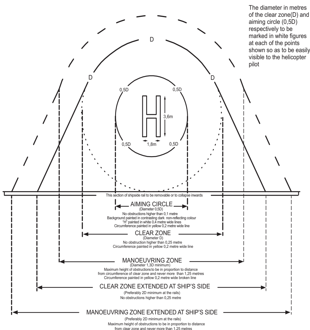
Figure 1 : Landing area at the ship's side
