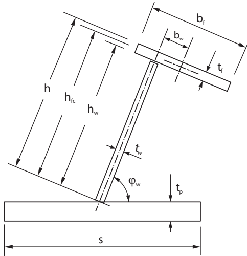
Figure 7 : Stiffener geometry
