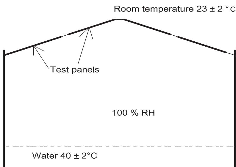
Figure 3 : Condensation chamber
