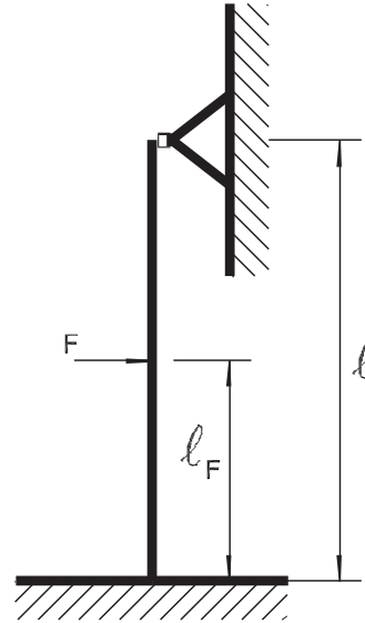
Figure 4 : Reference structure model
