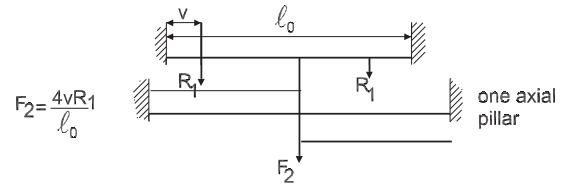
Figure 20 : Shear force diagram for elementary load [f] - Force F_2
