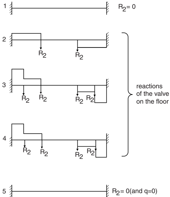
Figure 18 : Shear force diagram for elementary load [d] - Reactions R_2
