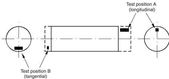
Figure 1 : Plain shaft
