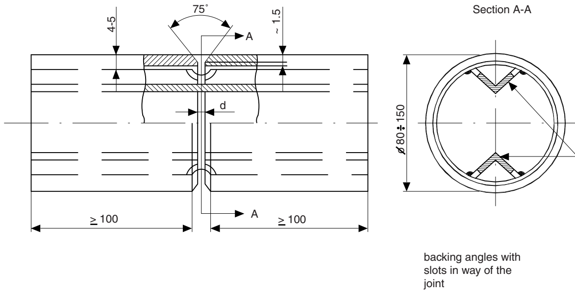
Figure 3 : Pipe assembly
