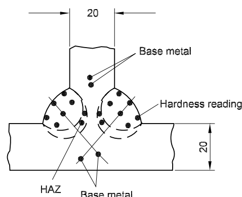
Figure 8 : Hardness readings
