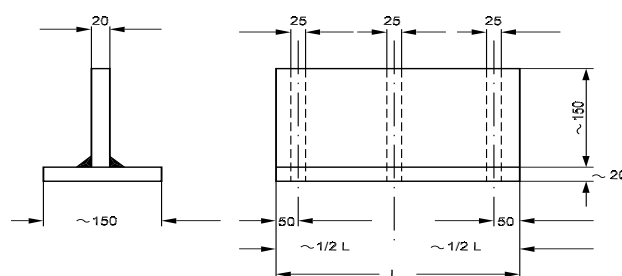
Figure 7 : Sections for micrographic examination
