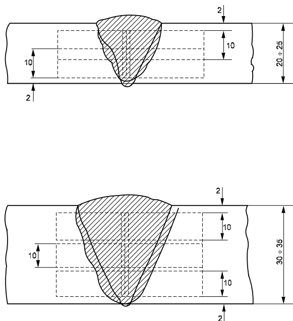
Figure 15 : Position of Charpy V-notch impact test for one side automatic welding
