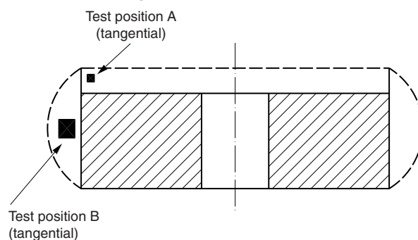
Figure 6 : Gear wheel
