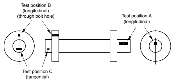
Figure 2 : Flanged shaft
