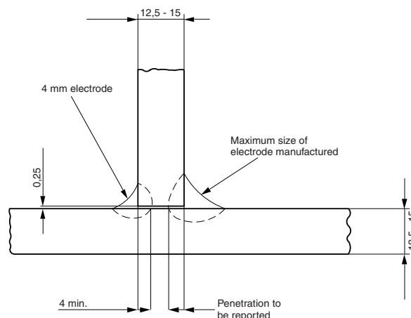
Figure 10 : Deep penetration fillet weld test assembly
