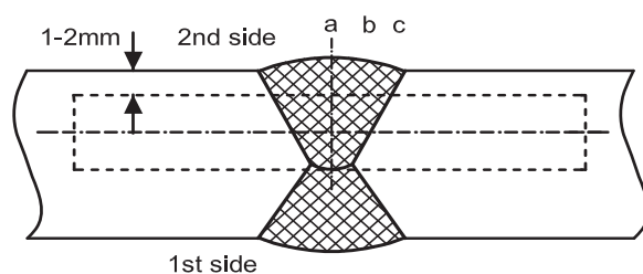
Figure 3 : Locations of V-notch for butt weld of normal heat input (heat input \leq 50 kJ/cm)
