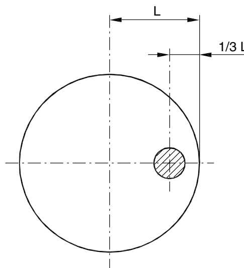
Figure 5 : Bars
