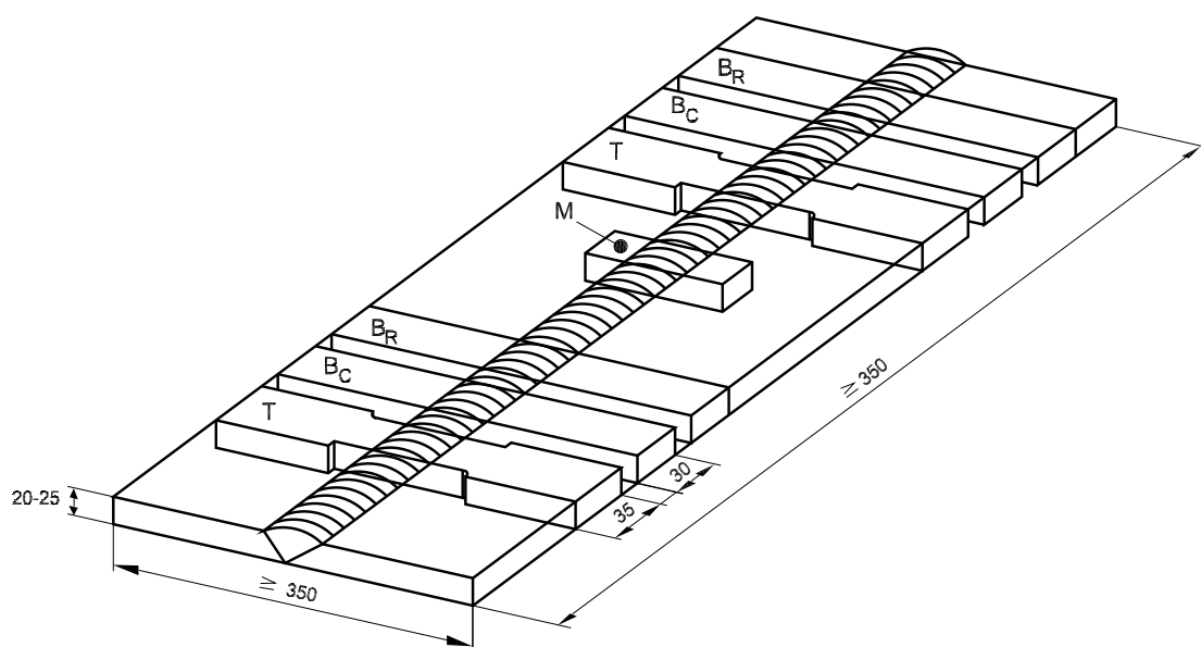
Figure 22 : Additional butt weld test assembly in downhand position
