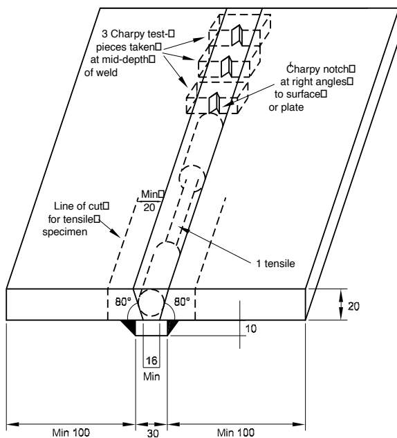
Figure 4 : Deposited metal test assembly
