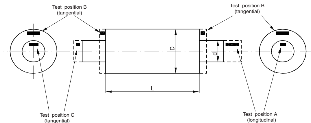
Figure 5 : Pinions
