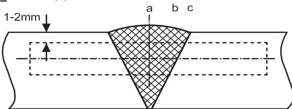
Figure 3 : Locations of V-notch for butt weld of normal heat input (heat input \leq 50 kJ/cm)
