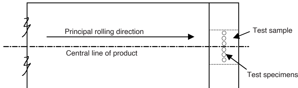
Figure 8 : Plate and wide flat sampling position
