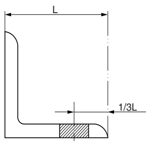
Figure 3 : Angles
