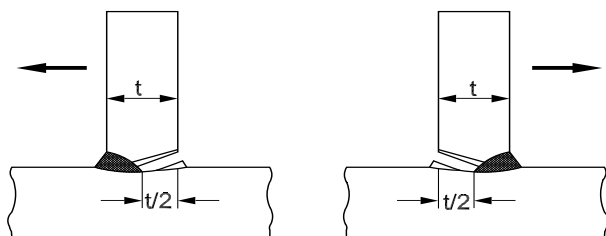
Figure 9 : Break test
