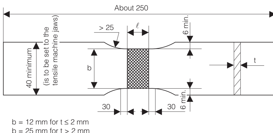
Figure 1 : Flat tensile test specimen
