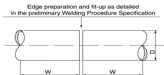
Figure 10 : Pipe weld test assembly
