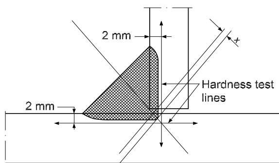
Figure 9 : Macro and hardness indentations
