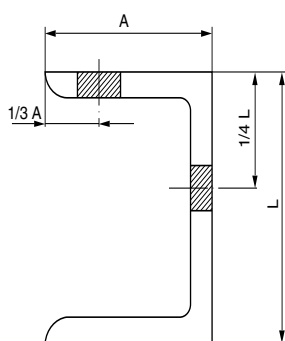
Figure 4 : Sections
