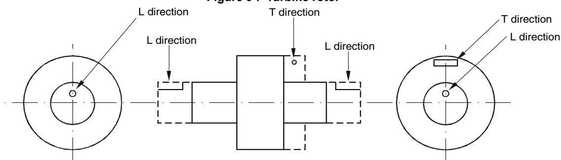
Figure 9 : Turbine rotor
