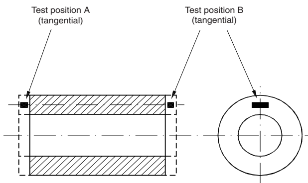
Figure 8 : Pinion sleeve
