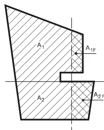
Figure 3 : Geometry of rudder blade with cut-outs
