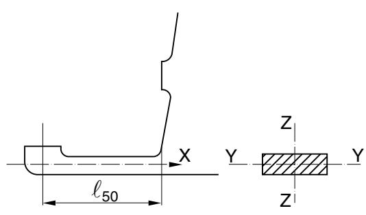
Figure 4 : Solepiece geometry
