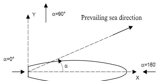
Figure 1 : Wave heading
