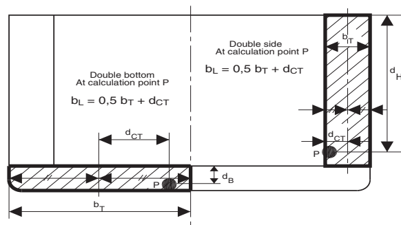
Figure 5 : Distances b_L and d_H
