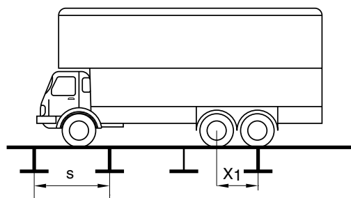
Figure 3 : Wheeled loads - Distance between axles of two consecutive vehicles
