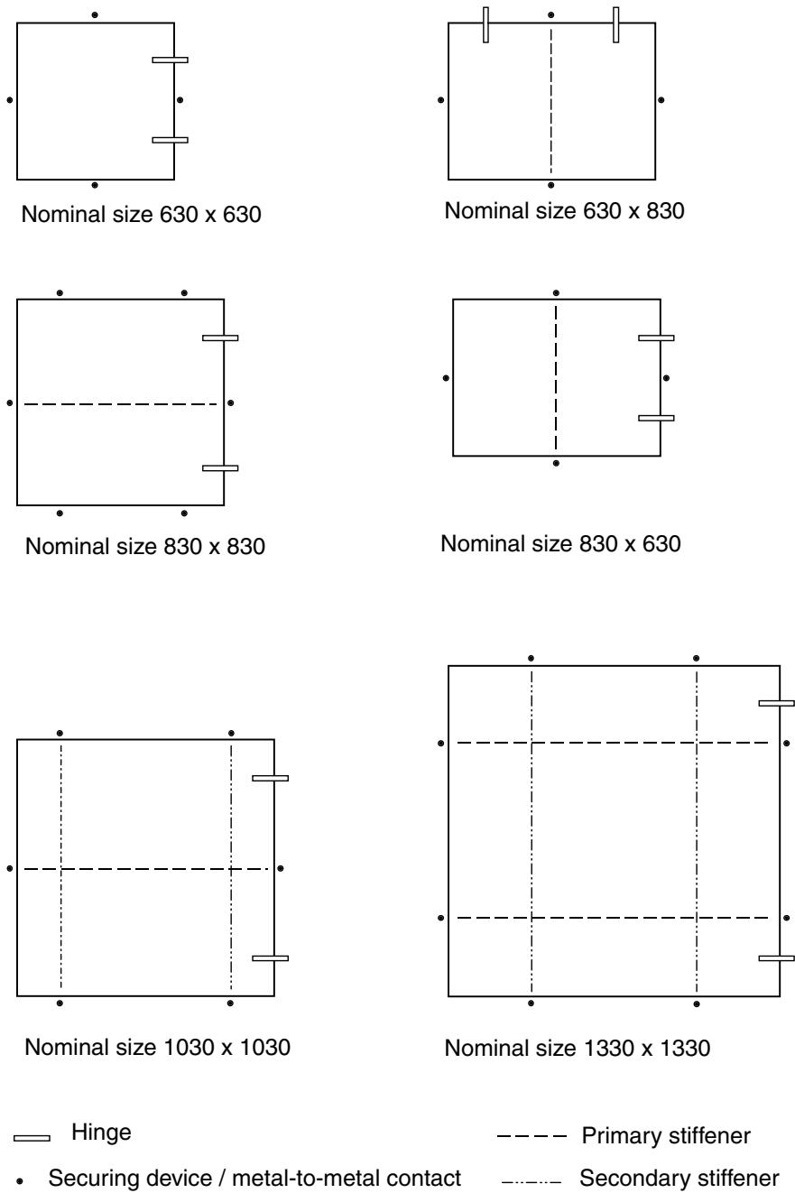
Figure 2 : Structural arrangement of small rectangular steel hatch covers
