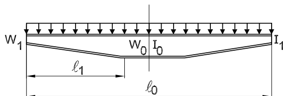
Figure 1 : Variable cross-section stiffener
