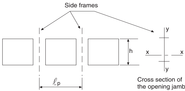
Figure 3 : Side openings
