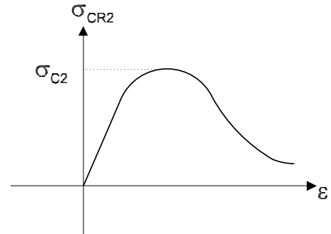
Figure 5 : Load-end shortening curve \sigma_{CR2}-\varepsilon for flexural-torsional buckling
