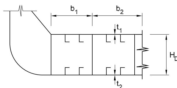
Figure 7 : Beams of double skin structures
