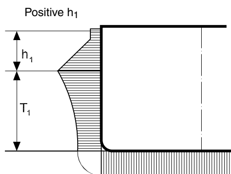
Figure 2 : Wave pressure in load case “a”
