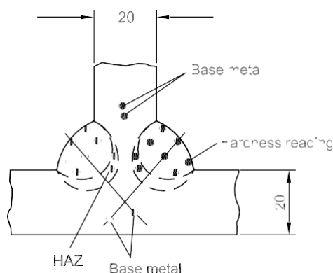
Figure 4 : Hardness readings
