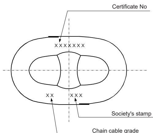
Figure 7 : Marking of chain cables
