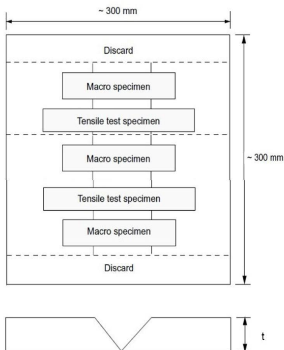
Figure 17 : Test Specimen for cast steel propellers
