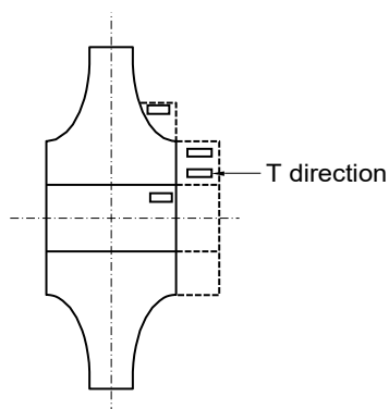
Figure 12 : Turbine disc
