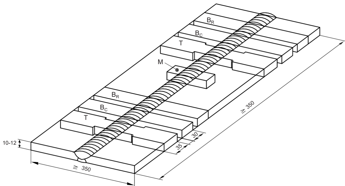
Figure 13 : Butt weld test assembly for positional welding
