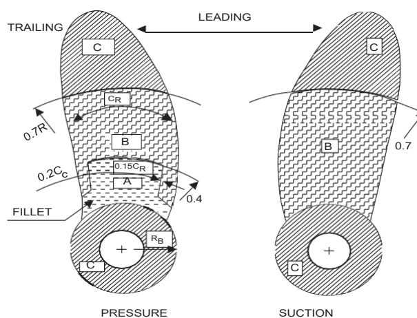
Figure 4 : Severity zones in blades with skew angles > 25°
