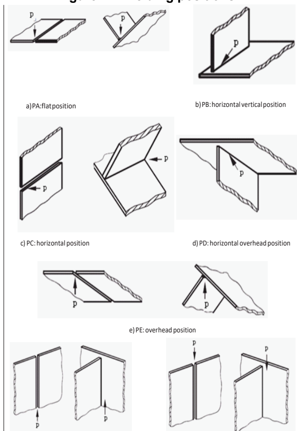
Figure 1 : Welding positions
