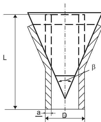
Figure 10 : Drift expanding test
