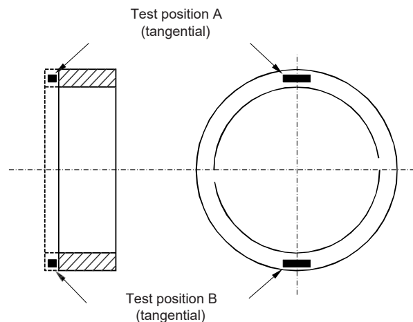
Figure 10 : Pinion sleeve
