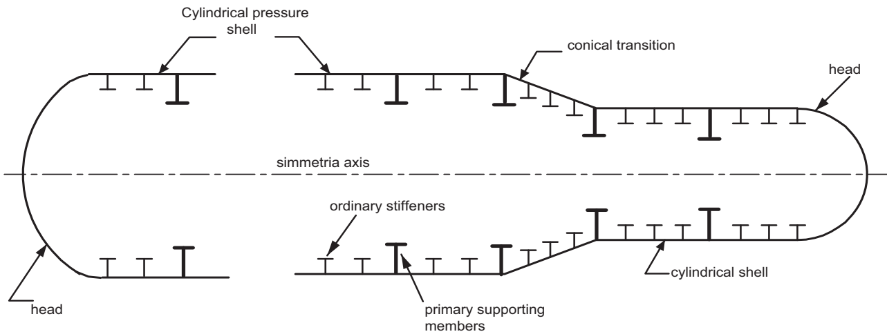
Figure 1 : Schematic plan of main structural components of a pressure shell
