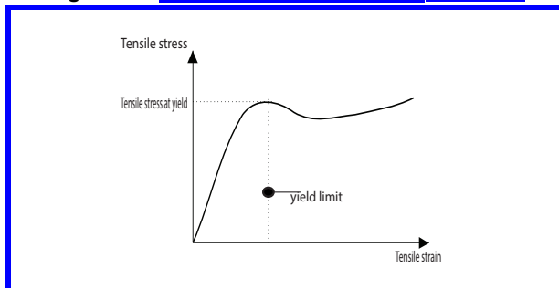
Figure 1 : Stress / elongation curve (1/5/2023)
