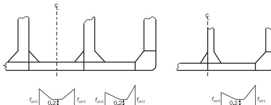
Figure 1 : Shear force distribution factors of floors
