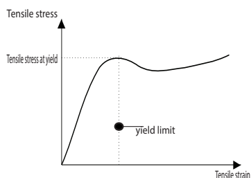
Figure 1 : Stress / elongation curve (1/5/2023)
