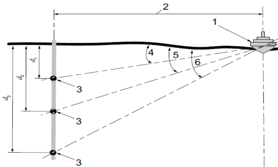
Figure 1 : Hydrophones geometry
