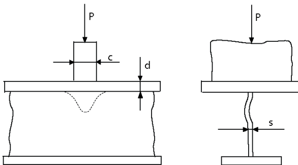
Figure 3: Local crippling
