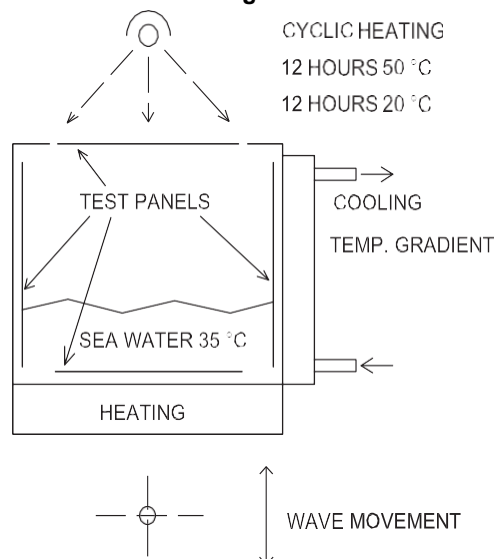
Figure 2 : Wave tank for testing of water ballast tank coating
