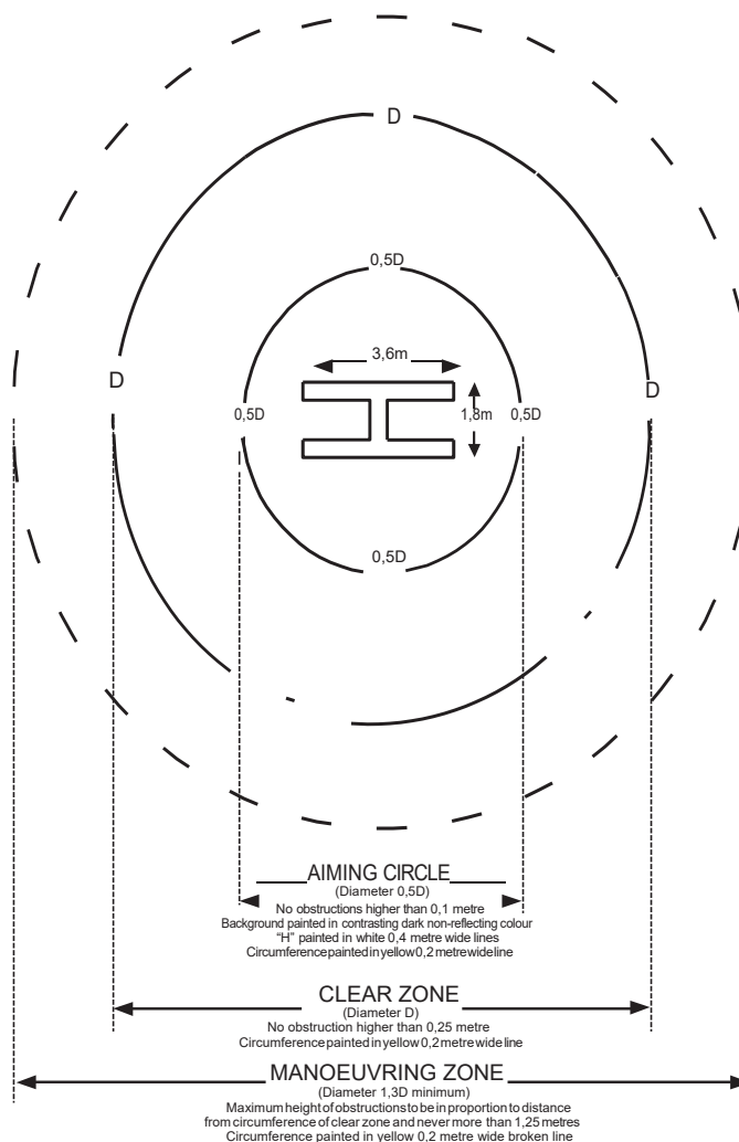
Figure 2 : Landing area without unobstructed access from ship's side (1/1/2012)
