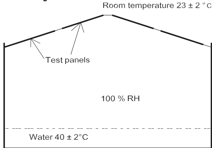
Figure 3 : Condensation chamber
