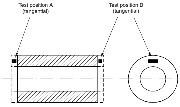
Figure 8 : Pinion sleeve
