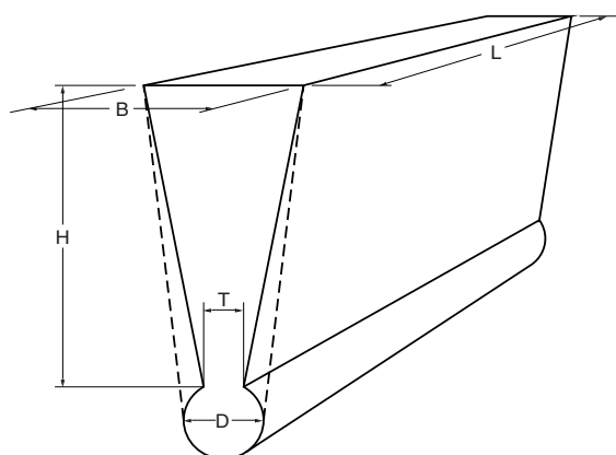
Figure 1 : Keel block test sample casting
