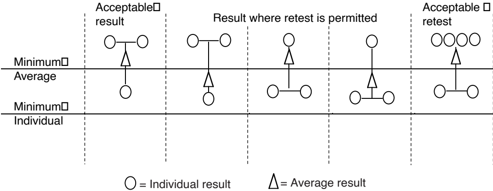
Figure 8 : Diagram showing acceptance / rejection and retest criteria
