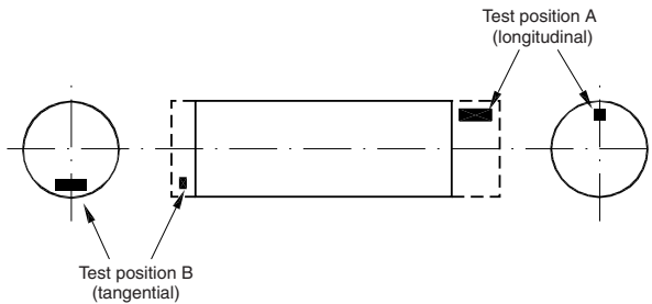
Figure 1 : Plain shaft
