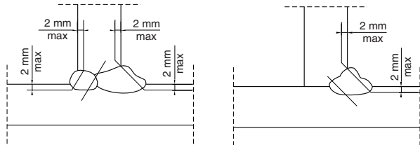
Figure 7 : Examples of hardness indentations
