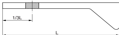
Figure 2 : Bulb flats
