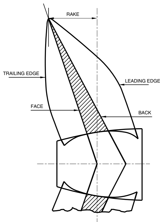
Figure 1 : Rake
