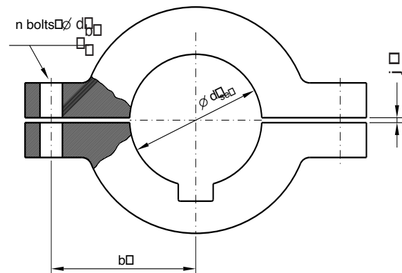
Figure 2 : Bolted tillers
