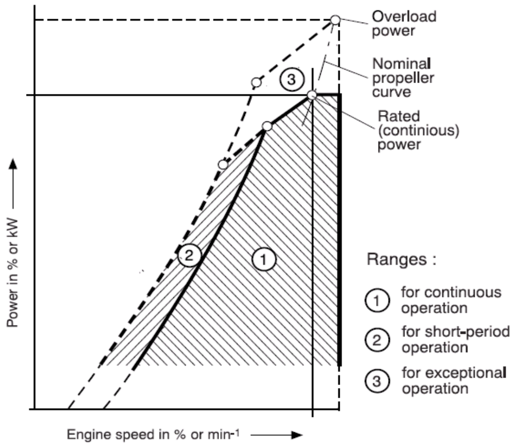
Figure 1 : Power/speed diagram
