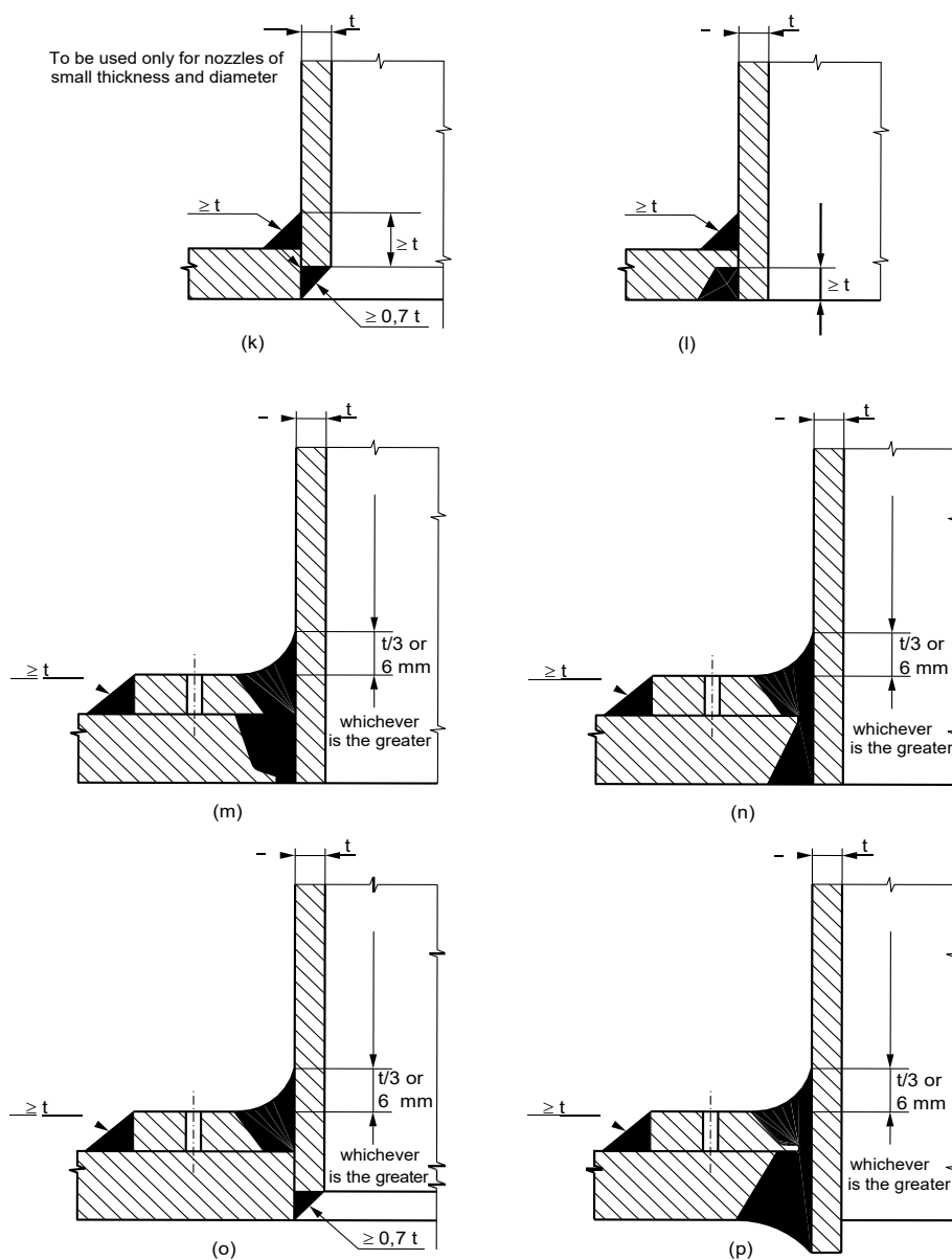
Figure 20 : Types of joint for nozzles and reinforcing rings (3)
