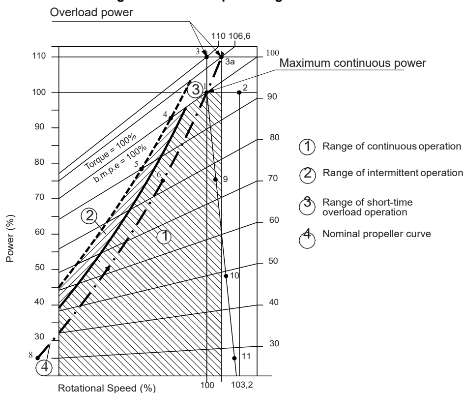
Figure 2 : Power/speed diagram
