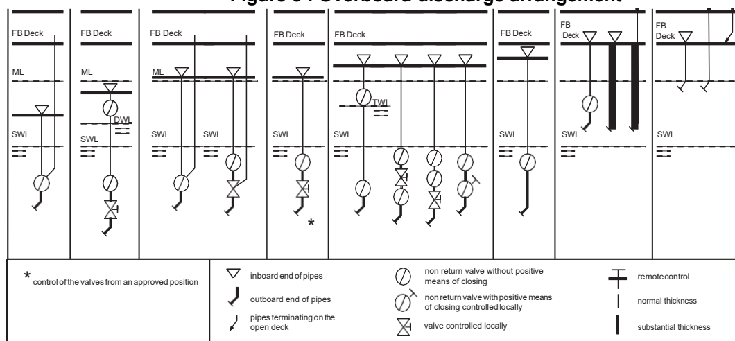
Figure 3 : Overboard discharge arrangement
