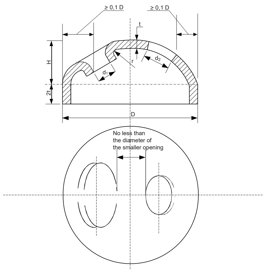
Figure 9 : Openings on dished heads
