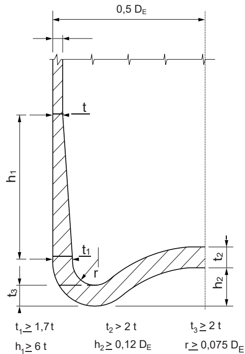
Figure 14 : Heads with openings
