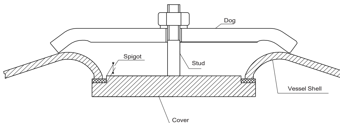
Figure 1 : Opening cover
