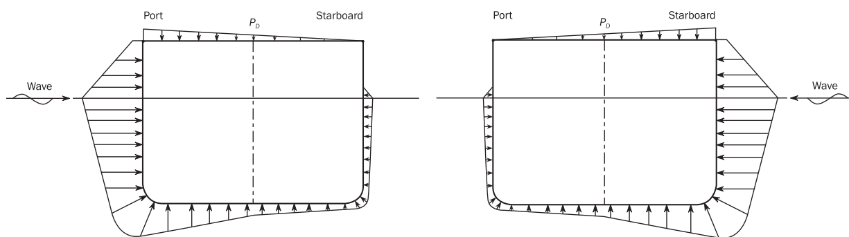
Figure 10 : Transverse distribution of dynamic pressure amidships for OSA-1P (left) and OSA-1S (right) load cases
