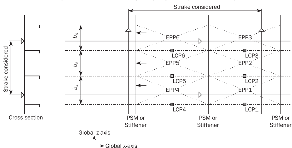
Figure 18 : Load calculation point (LCP) for longitudinal framing
