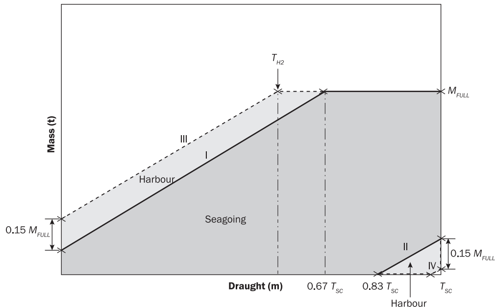
Example BC-B and BC-C ships not having {No MP}
