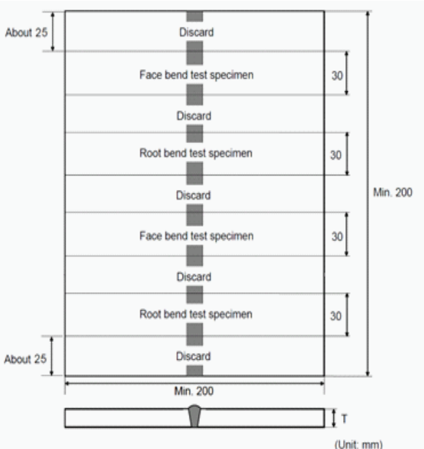
Figure 2 : Dimensions and types of test assembly for butt welds (T < 12mm) (1/1/2018)
