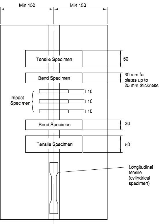
Figure 7 : Butt weld test assembly (1/7/2019)
