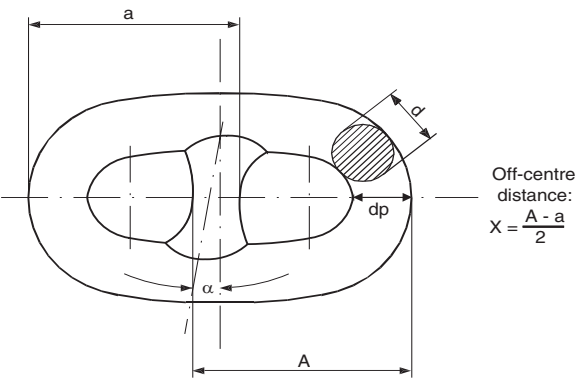
Figure 6 : Manufacturing tolerances
