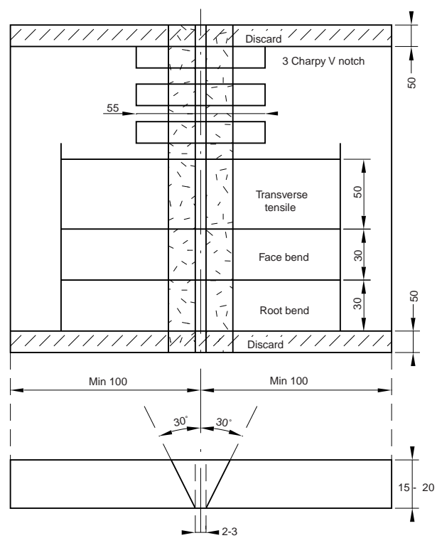
Figure 2 : Buttt weld test assembly (1/7/2019)
