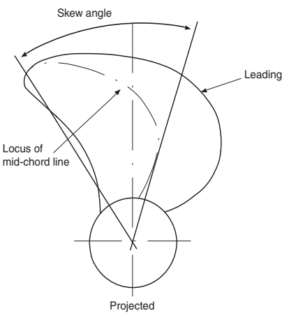
Figure 2 : Definition of skew angle
