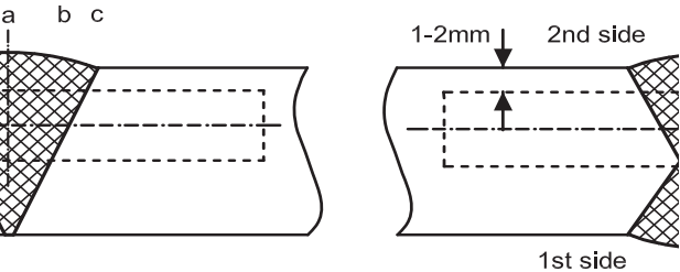
Figure 3 : Locations of V-notch for butt weld of normal heat input (heat input £ 50 kJ/cm) (1/1/2007)
