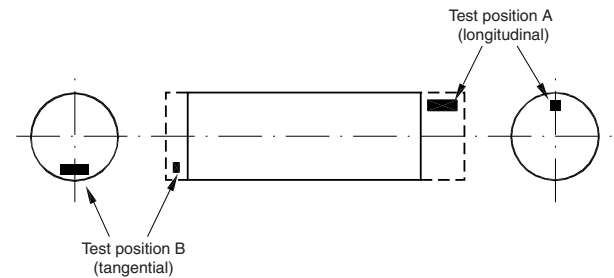
Figure 2 : Plain shaft
