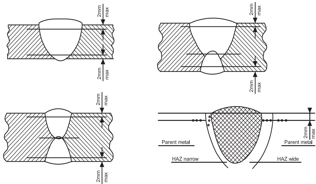
Figure 5 : Examples of hardness indentations (1/1/2007)
