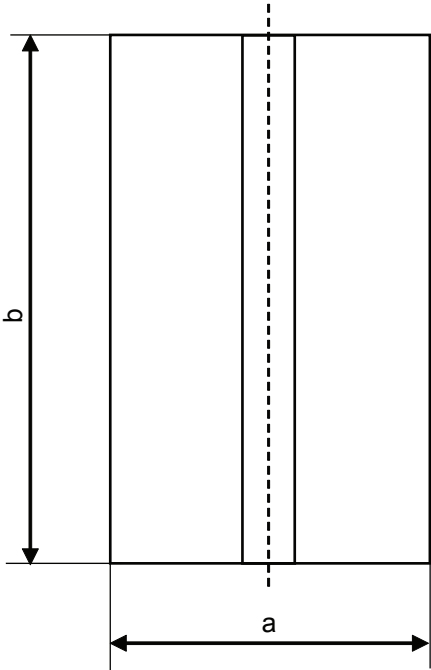
Figure 8 : T fillet joint on plate (1/1/2015)
