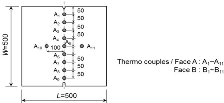
Figure 4 : Locations of temperature measurement (1/1/2021)
