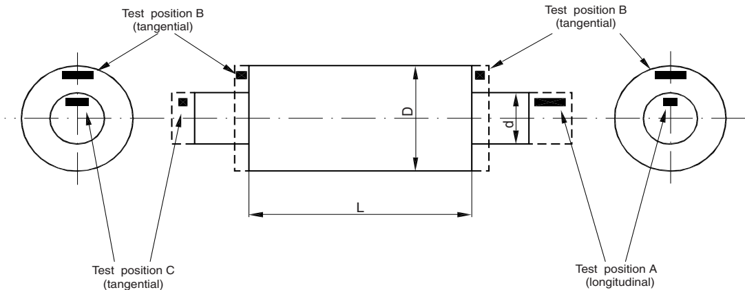
Figure 7 : Pinions
