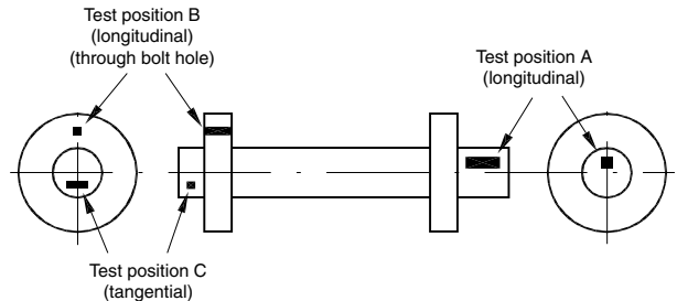
Figure 3 : Flanged shaft
