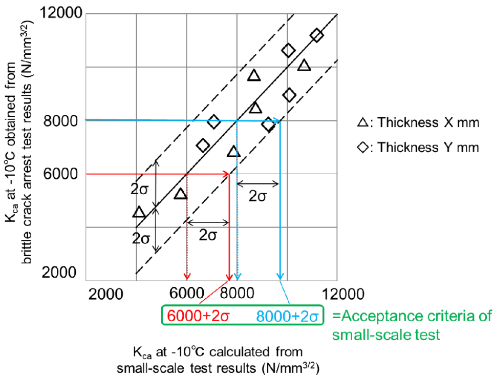
Figure 2 : Example for determination of acceptance criteria of small-scale test for correlation by means of brittle crack arrest toughness ( K_{ca} ) (1/7/2024)
