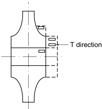
Figure 12 : Turbine disc
