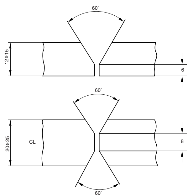
Figure 9 : Recommended edge preparation for two-run butt weld test assemblies (1/7/2019)
