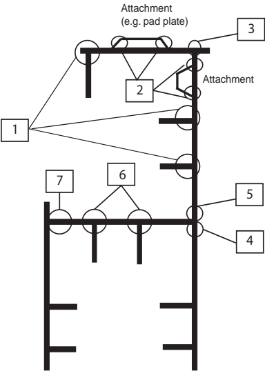
Figure 13 : Other Weld Areas (1/1/2017)
