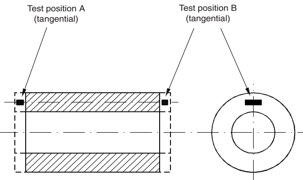
Figure 10 : Pinion sleeve
