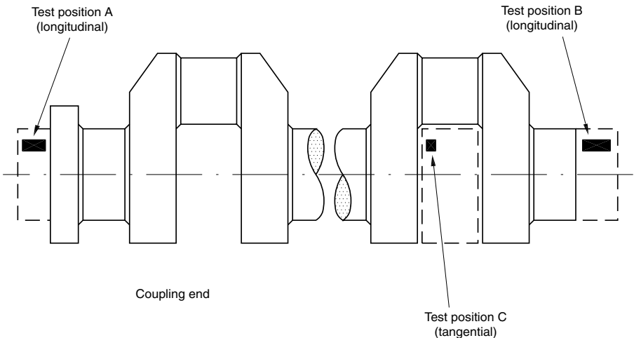
Figure 5 : Solid forged crankshaft
