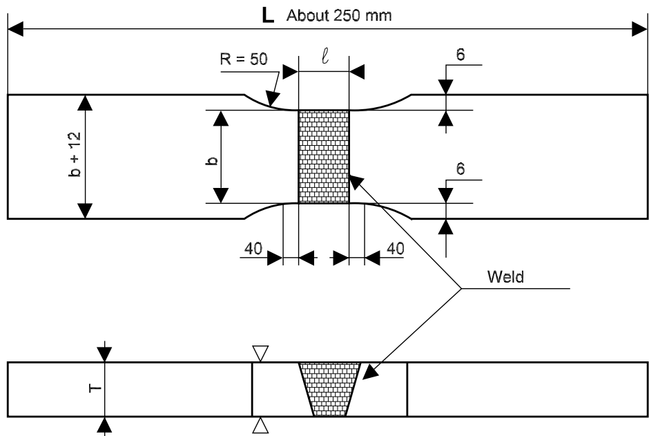
Figure 12 : Transverse tensile specimen
