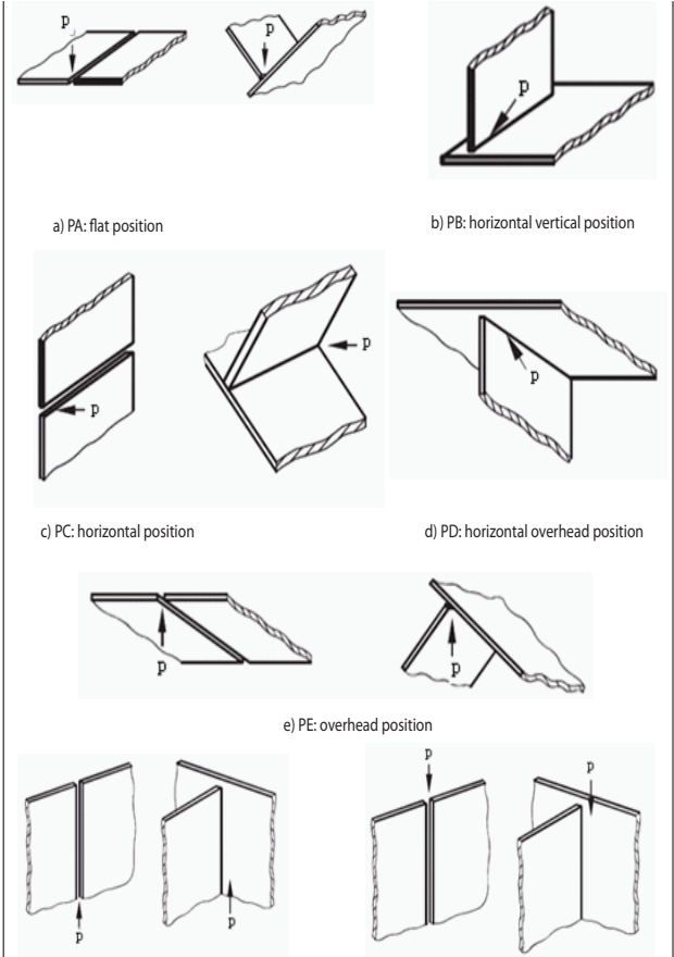
Figure 1 : Welding positions
