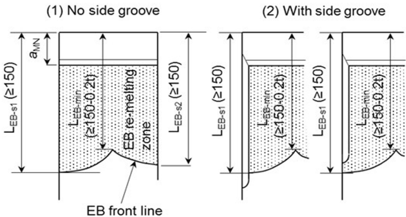
Figure 3 : Definition of EBW length (1/1/2021)
