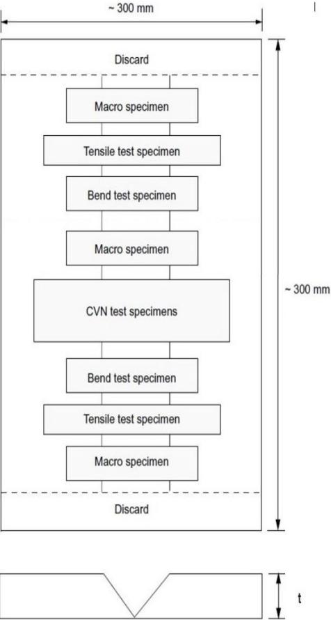
Figure 16 : Test Specimen for cast steel propellers (1/7/2021)
