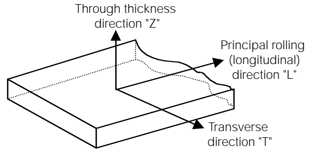
Figure 9 : Normal test specimen (1/7/2003)
