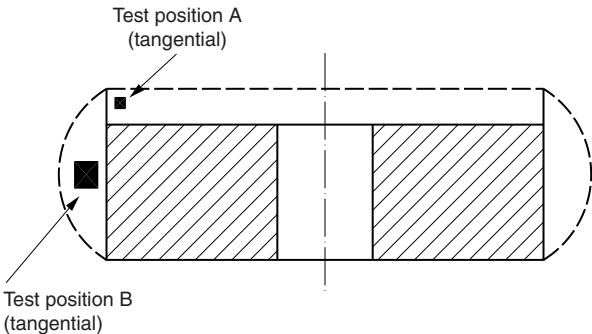
Figure 8 : Gear wheel
