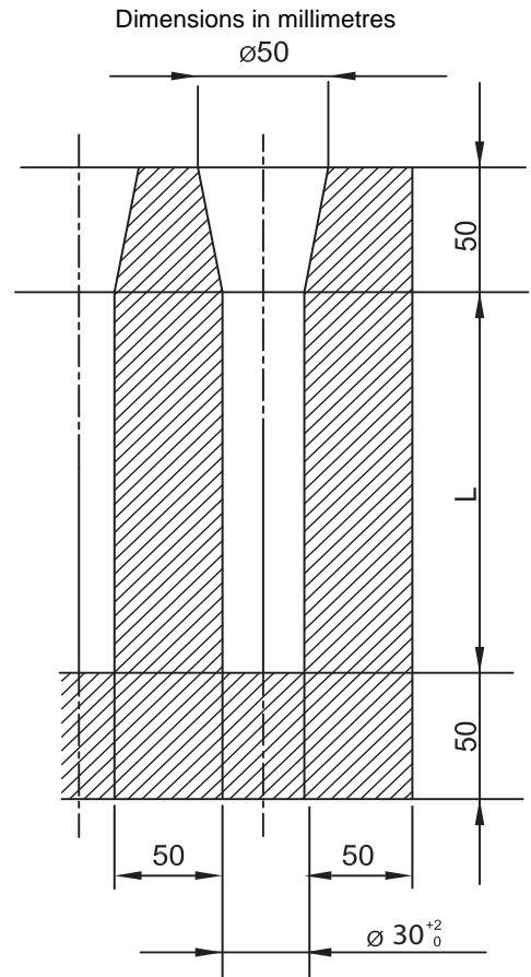
Figure 1 : Test Sample for grey cast iron
