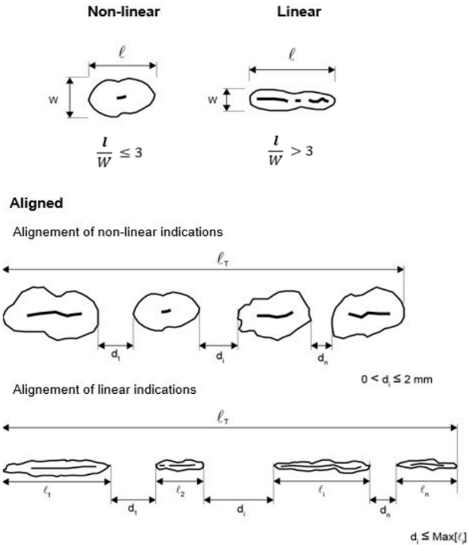
Figure 7 : Shape of indications (1/1/2025)
