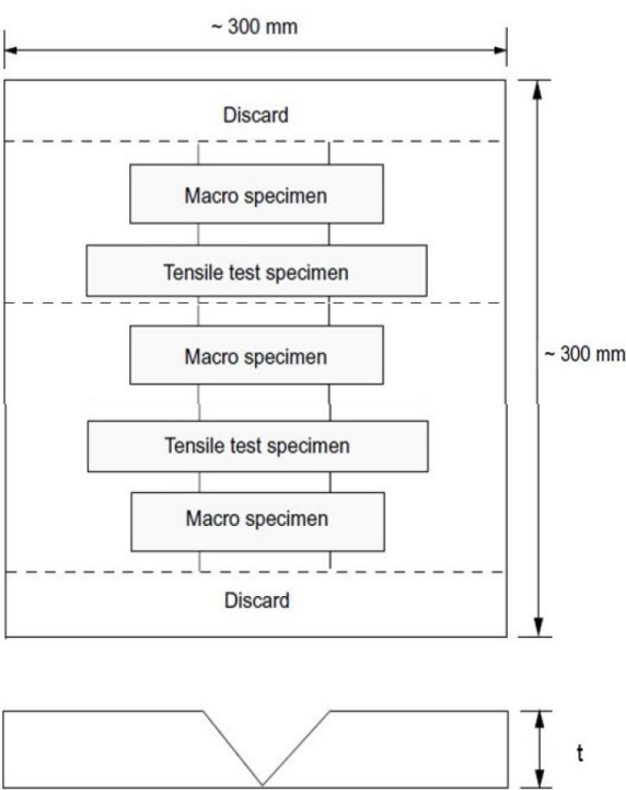
Figure 15 : Test Specimen for cast copper alloy propellers (1/7/2021)
