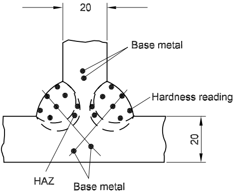
Figure 4 : Hardness readings (1/7/2019)
