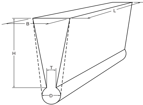
Figure 1 : Keel block test sample casting (1/1/2025)
