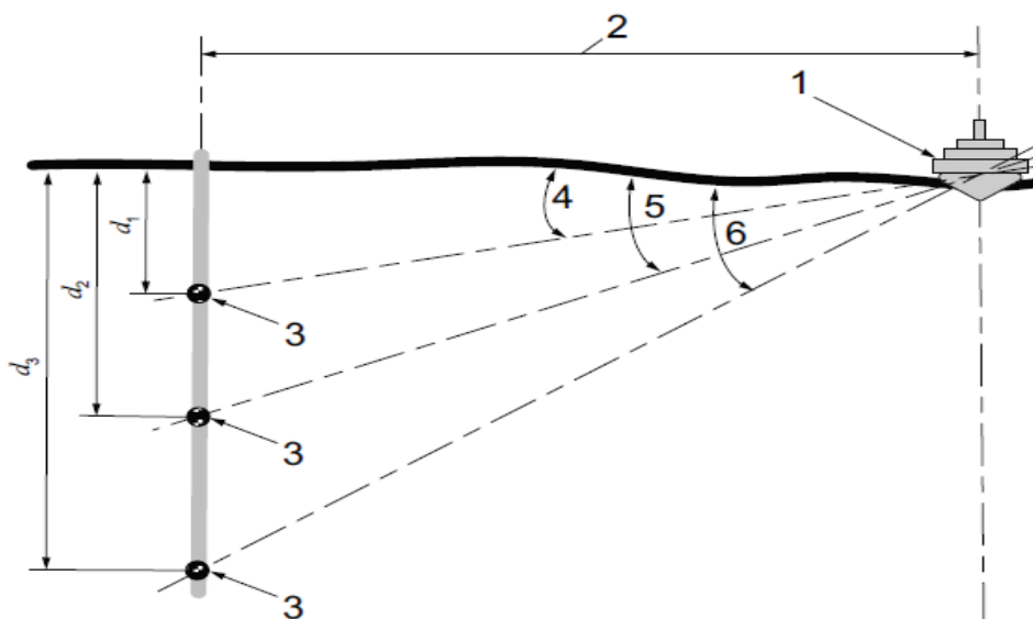
Figure 1 : Hydrophones geometry
