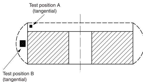
Figure 8 : Gear wheel
