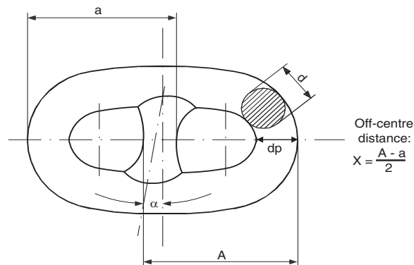
Figure 6 : Manufacturing tolerances
