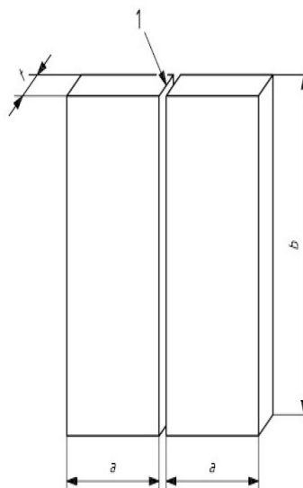
Figure 15 : Test piece for welding repair procedure for cast steel propellers
