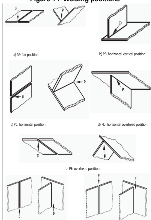
Figure 1 : Welding positions
