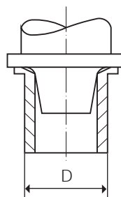
Figure 11 : Flanging test
