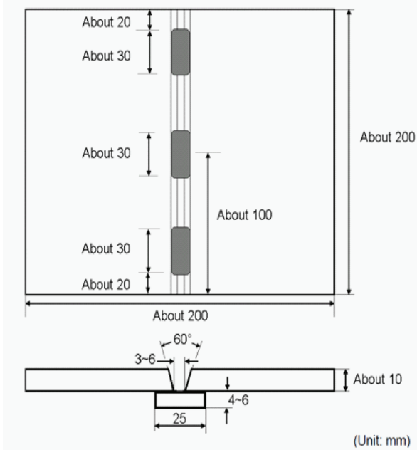
Figure 5 : Dimensions and types of test assembly for tack butt welds
