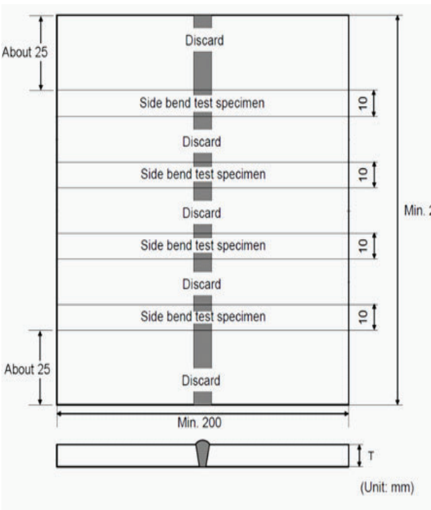
Figure 3 : Dimensions and types of test assembly for butt welds (T > 12mm)
