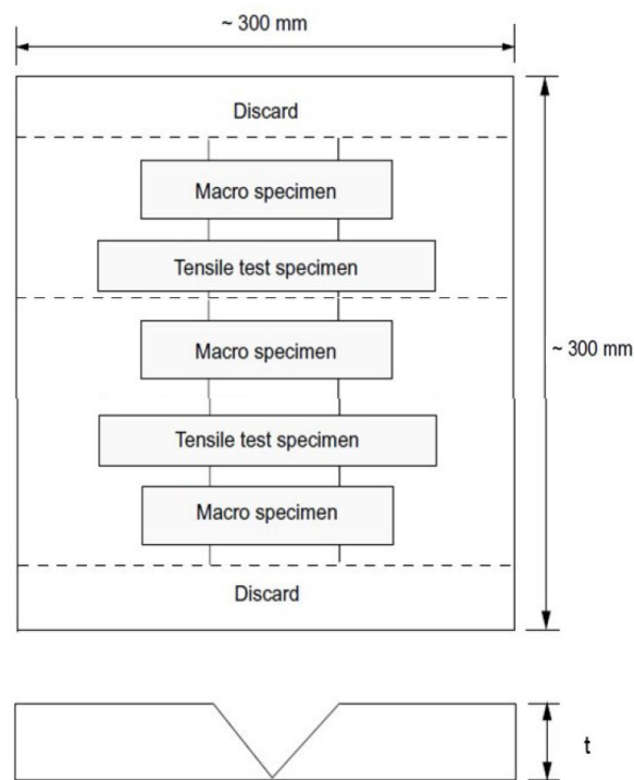
Figure 16 : Test Specimen for cast copper alloy propellers
