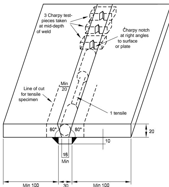
Figure 1 : Deposited metal test assembly
