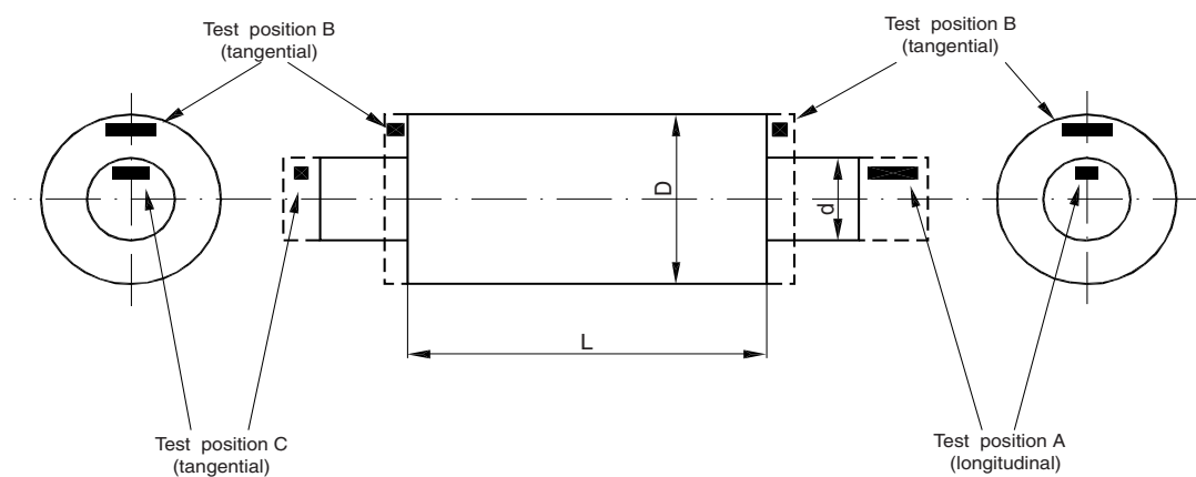
Figure 7 : Pinions
