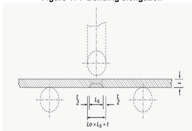
Figure 11 : Bending elongation
