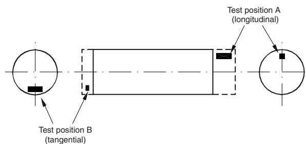
Figure 2 : Plain shaft
